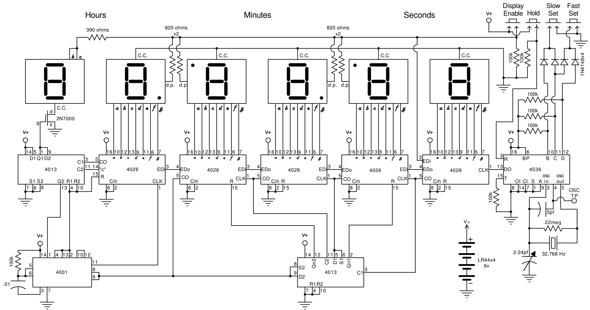
12 Hour 6 Digit LED Watch © 2010 Oldradiobuilder.com
